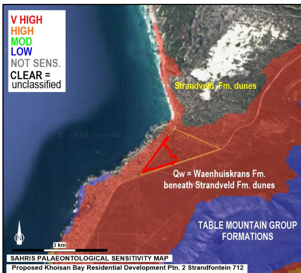
Figure 7. Palaeontological sensitivities of formations in the De Kelders area.
