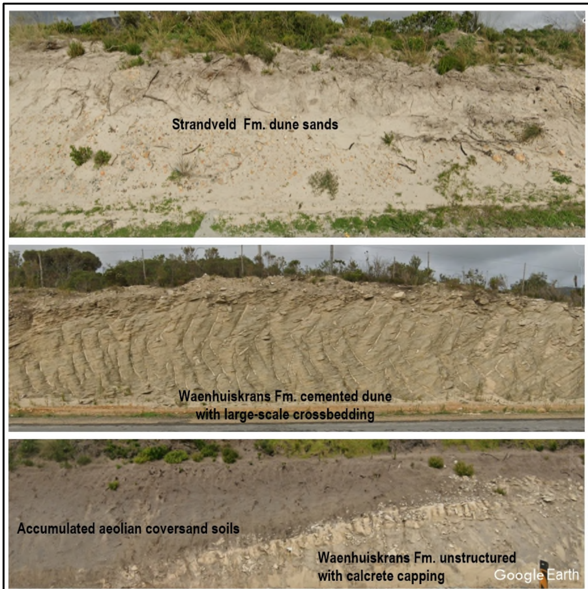
Figure 5. Exposures of the underlying geology in road cuttings along the R43 between Stanford and De Kelders.
