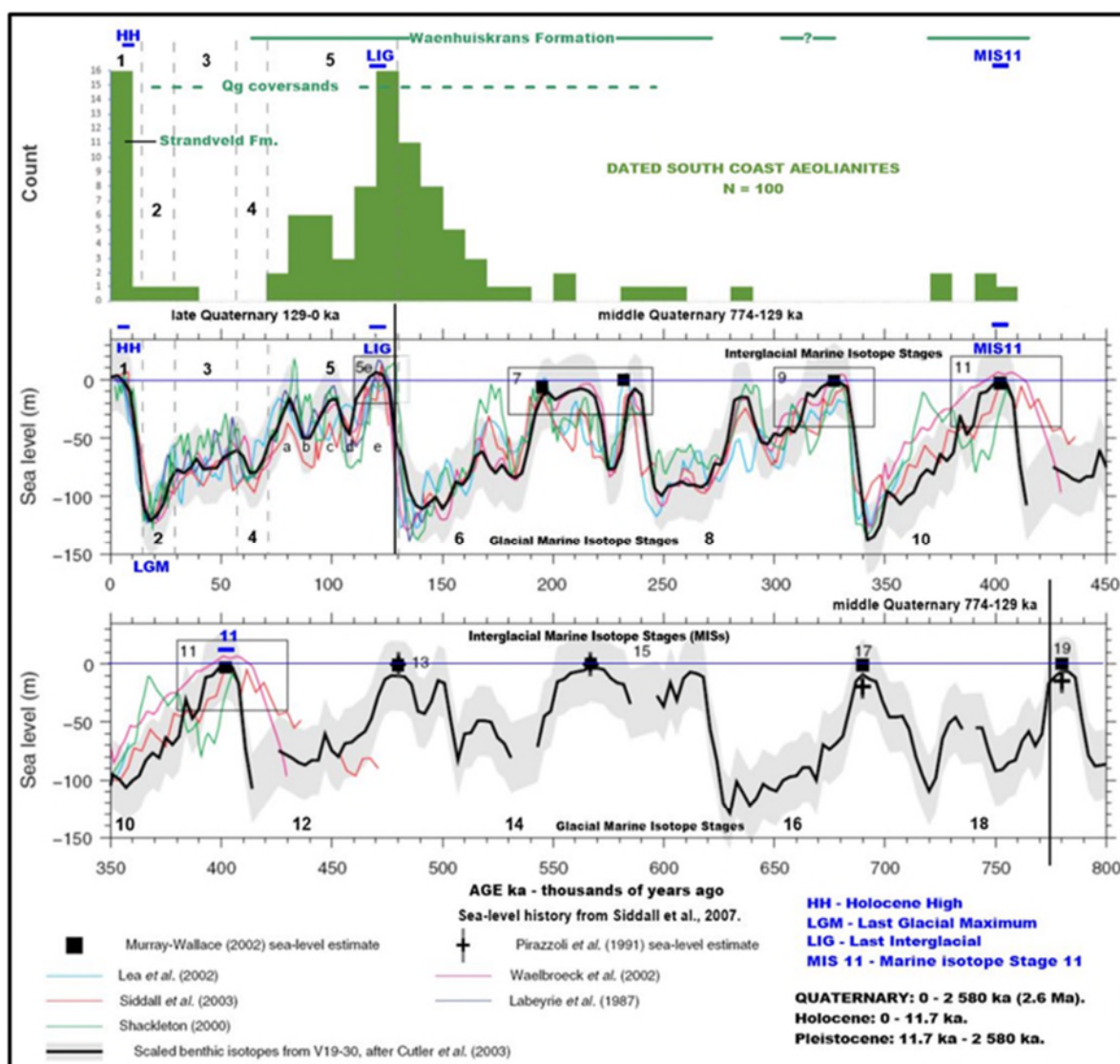
Figure 4. Sea-level history for the last 800 ka with numbered Marine Isotope Stages showing the ages of the Klein Brak Formation raised beaches and OSL dates from South Coast aeolianites.
