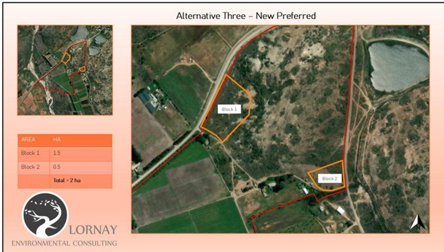
Figure 1: Proposed site layout plan (Alternative 3)
