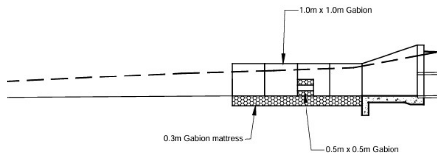
SECTION SCALE 1:100
