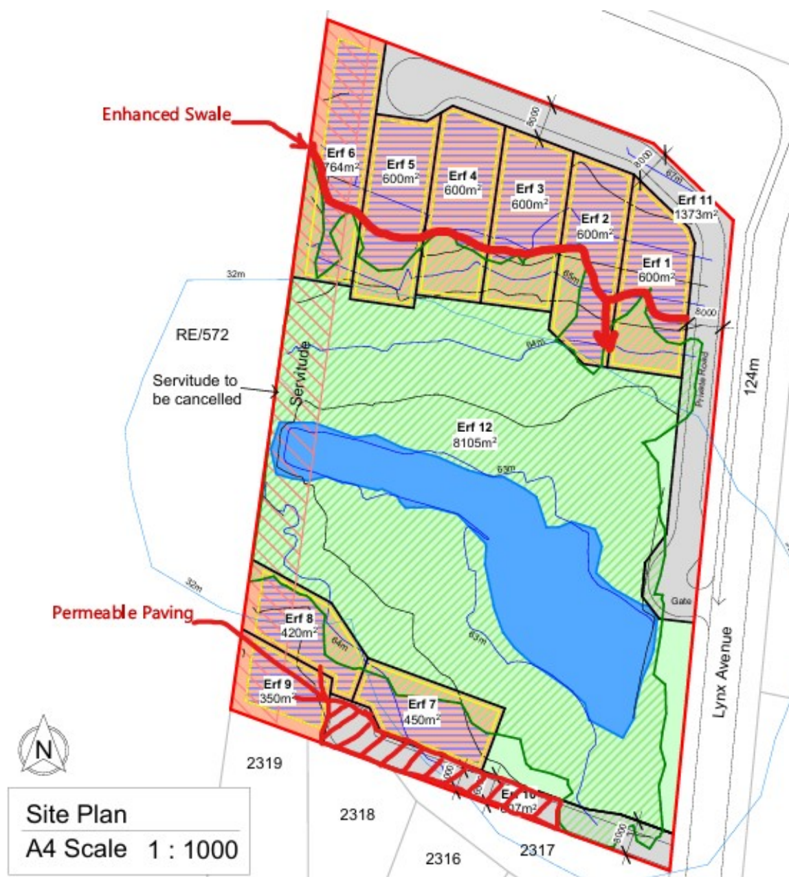
Drawing 4 -Proposed location of Permeable Paving and Enhanced Swale
