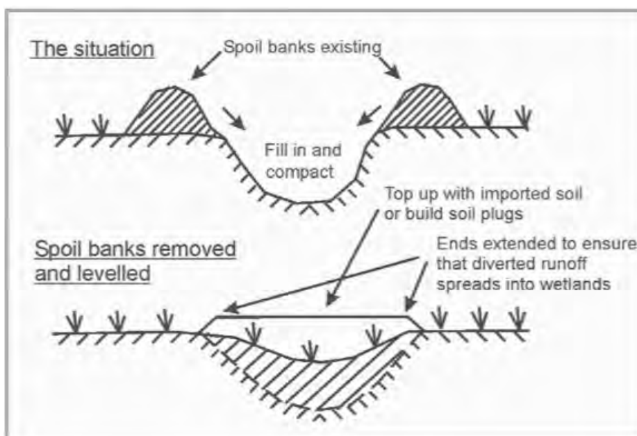
Figure 8-2: Sloping wetland banks.
