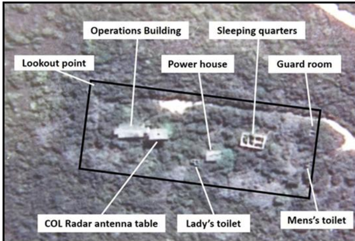
Figure 14 Layout of the buildings on the L'Agulhas Radar site.
