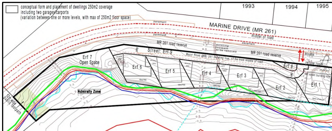
Figure 4. Preferred Site Development Plan. Umsiza Planning - 13 OCT. 2025.
