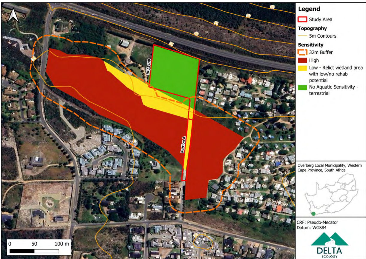
Figure 7-2: Aquatic sensitivity.
