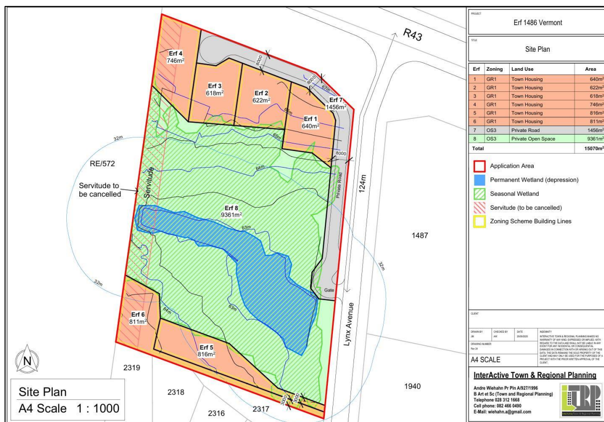
Figure 3. Development layout for Erf 1486, Vermont (Alternative 4).
