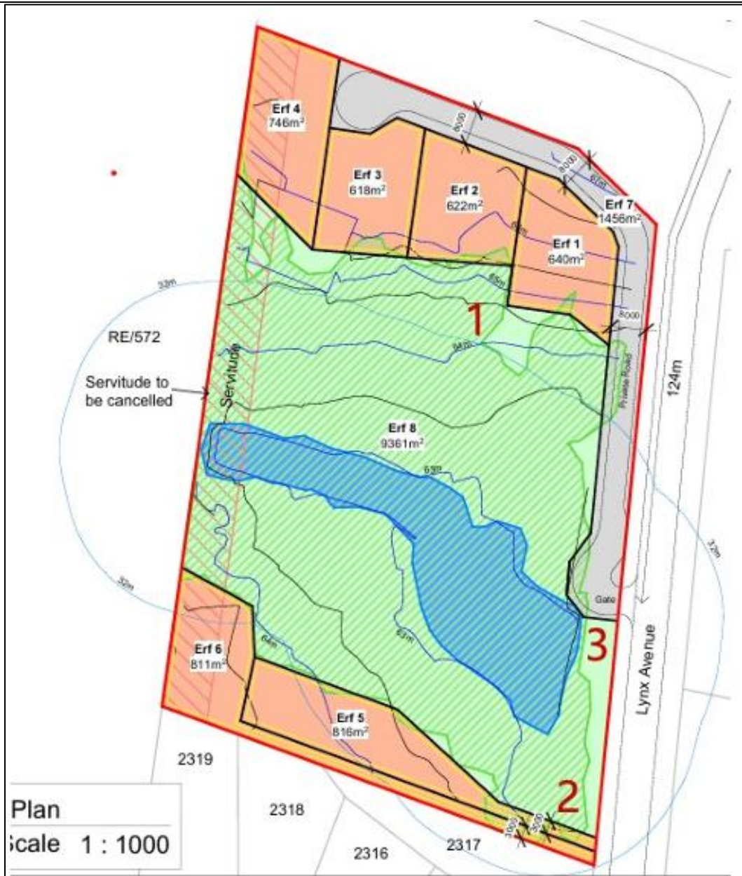
Figure 16b: Showing the position of the outlet's structures.
