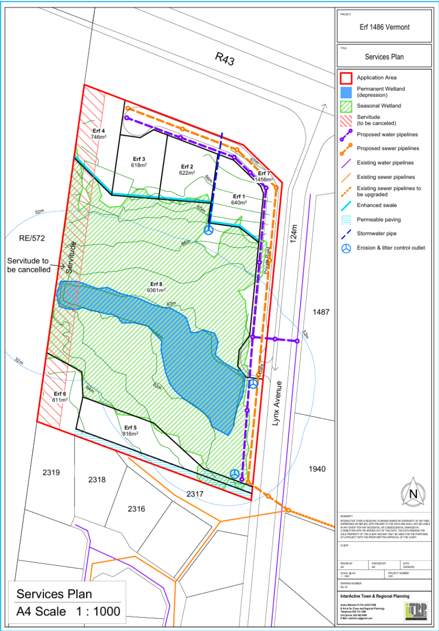
Figure 1b: Site development plan showing the stormwater swale and stormwater outlets as well as the service infrastructure alignment.
